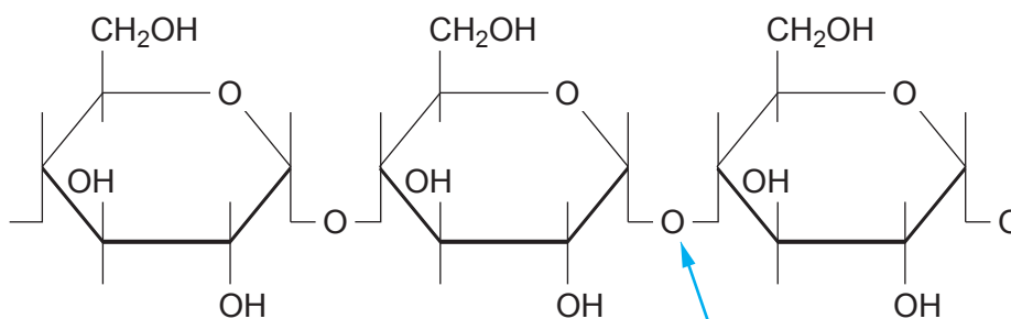
Amylose
