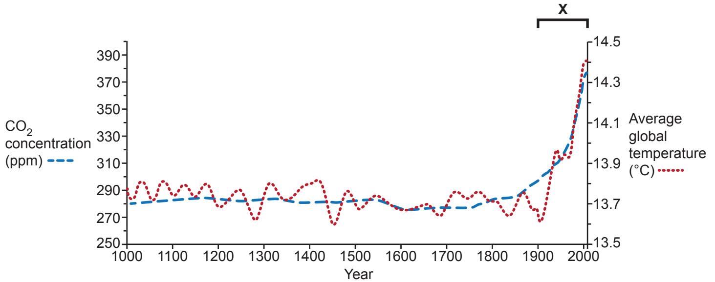
Fig. 4 Changes in global temperatures and carbon dioxide (CO 2 ) levels since 1000AD
