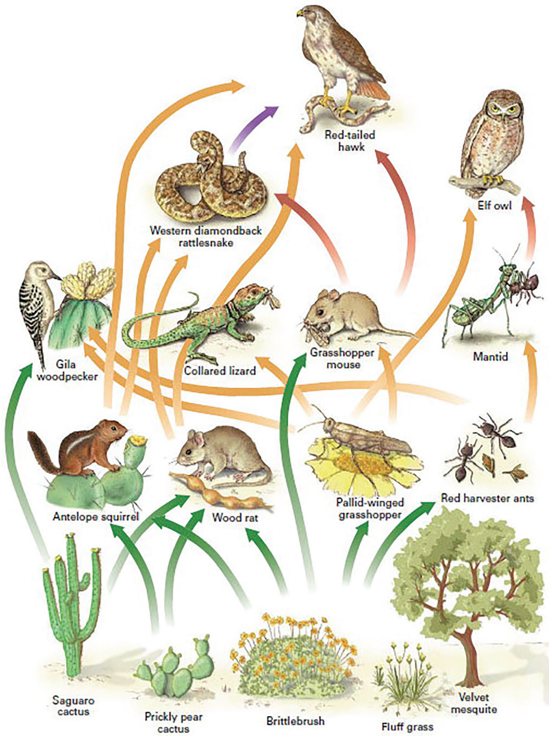
Fig. 1 Part of a hot desert ecosystem
